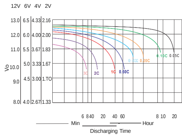
Discharging Characteristics@25°C(77°F)
